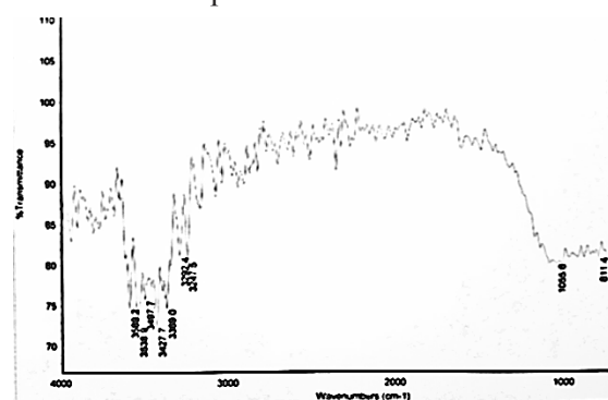
FTIR spectra of AC-nGO-bTiO2
