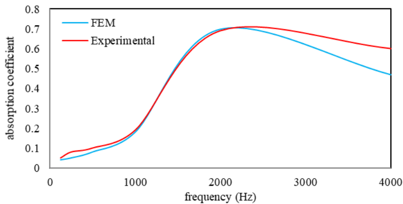
Fig. 2. Comparison between the results of sound absorption performance of experimental method and FEM
