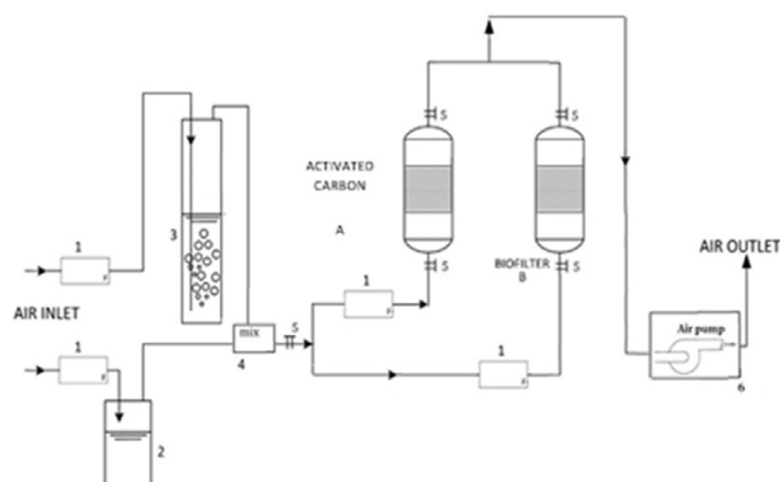
Fig. 1. Biofiltration System
