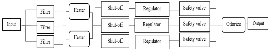
Fig. 2: Main subsystems of the CGS
