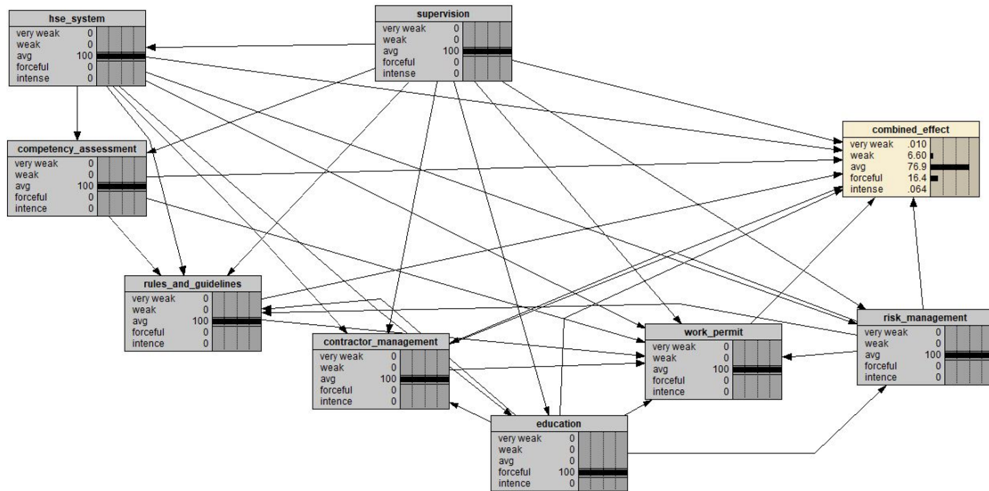
Fig. 1: BN created for the combined effect node.
